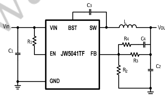
3.3V/2A Step-down Regulator
