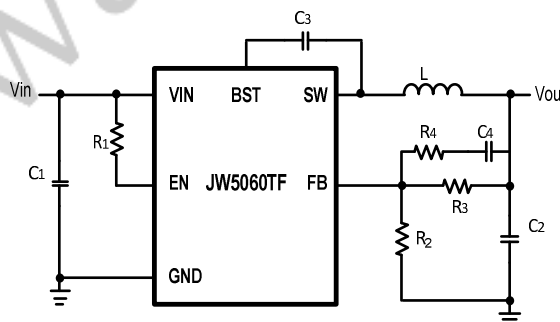
3.3V/3A Step-down Regulator
