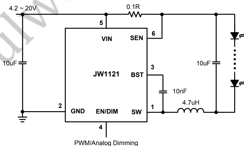
1A Buck LED Driver
